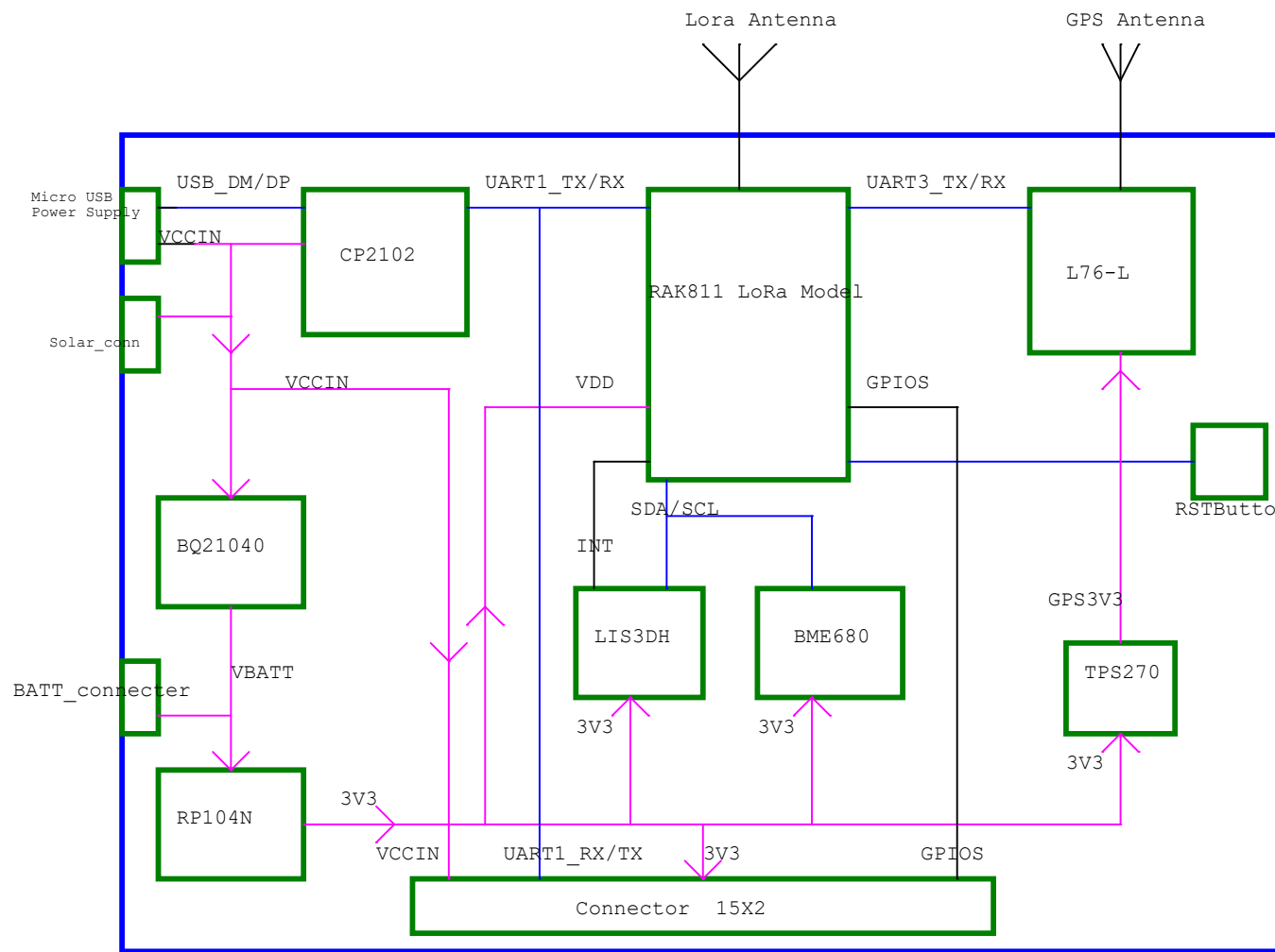
Block diagram
